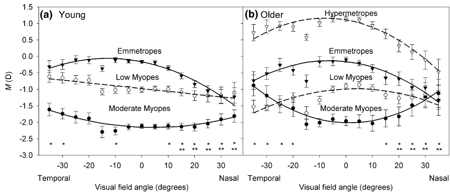
Fig. 1. Mean spherical equivalent refraction M as a function of visual field angle for each of the refractive subgroups for (a) young subjects and (b) older subjects. Errors bars indicate \pm SE (some are not seen where they are similar to size of symbols). Visual field points marked with an asterisk are those for which the differences between peripheral and central M are significantly correlated with central mean spherical equivalent refraction ( M ). A single asterisk indicates p < 0.05 and double asterisks indicate p < 0.004 (Bonferoni correction applied). Curve fits coefficients are shown in Table 2. The result for 15° temporal field appears in the figure, but was not used in curve calculations.
