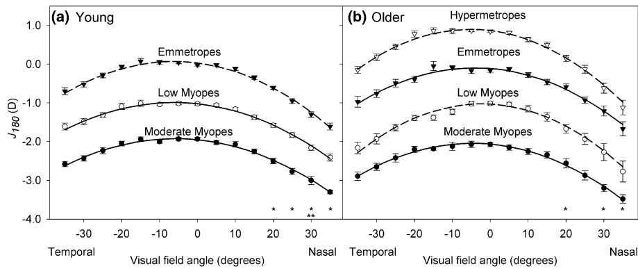
Fig. 2. Mean J_{180} astigmatism as a function of visual field angle for each of the refractive subgroups for (a) young subjects and (b) older subjects. Errors bars indicate \pm SE (some are not seen where they are similar to size of symbols). Visual field points marked with an asterisk are those for which the differences between peripheral and central J_{180} are significantly correlated with central mean spherical equivalent refraction ( M ). A single asterisk indicates p < 0.05 and double asterisks indicates p < 0.004 (Bonferoni correction applied). Results for hypermetropes, low myopes and moderate myopes (and the corresponding fitted curves) have been offset vertically for clarity by +1 D, -1 D and -2 D, respectively. Curve fit coefficients before the offsets are shown in Table 2. The result for 15° temporal field appears in the figure, but was not used in curve calculations.
