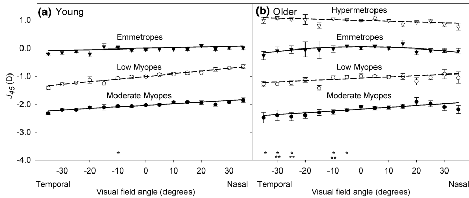
Fig. 3. Mean J_{45} astigmatism as a function of visual field angle for each of the refractive subgroups for (a) young subjects and (b) older subjects. Errors bars indicate \pm SE (some are not seen where they are similar to size of symbols). Visual field points marked with an asterisk are those for which the differences between peripheral and central J_{45} are significantly correlated with central mean spherical equivalent refraction ( M ). A single asterisk indicates p < 0.05 and double asterisks indicates p < 0.004 (Bonferroni correction applied). Results for hypermetropes, low myopes and moderate myopes (and the corresponding fitted curves) have been offset vertically for clarity by +1 D, -1 D and -2 D, respectively. Curve fit coefficients before the offsets are shown in Table 2. The result for 15° temporal field appears in the figure, but was not used in curve calculations.
